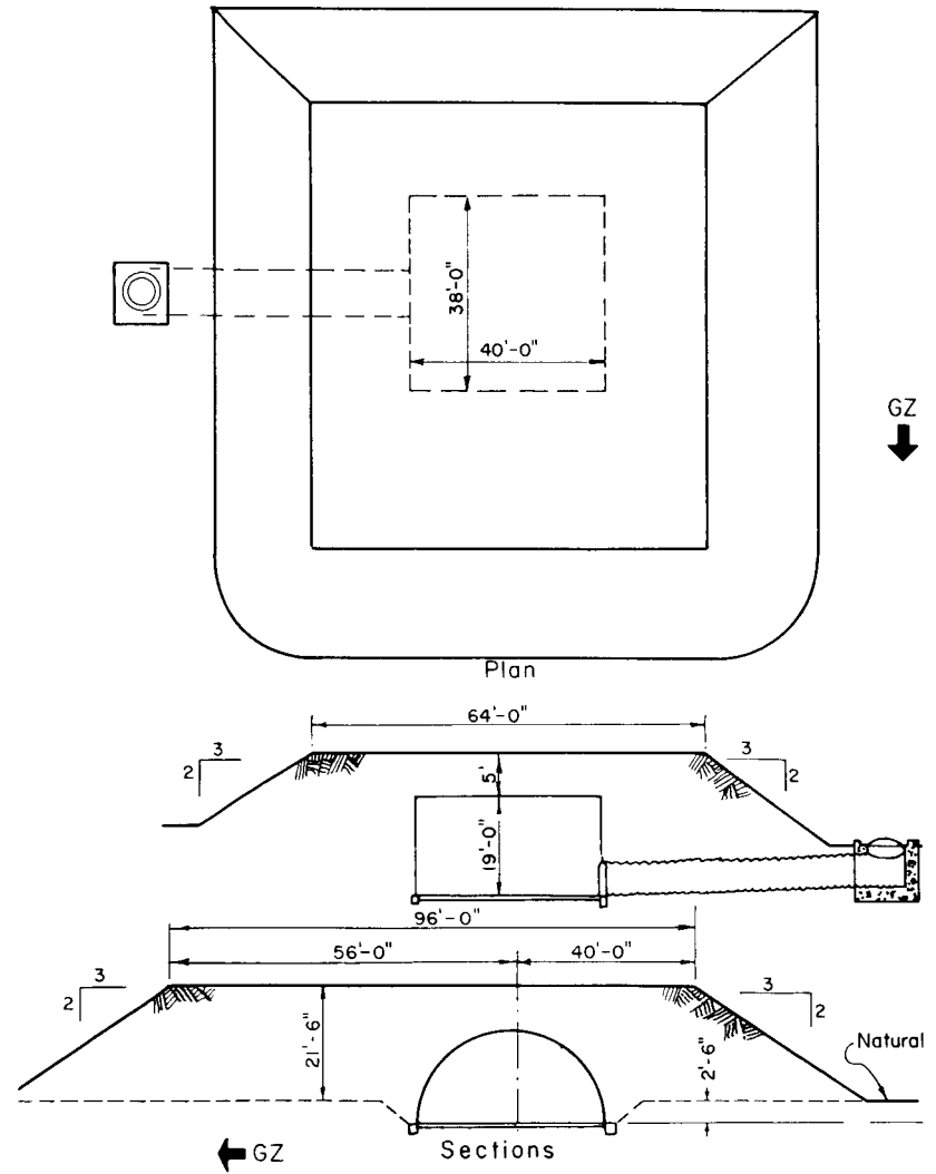
Fig. 9—Earth configuration, 38-ft-span structure.
